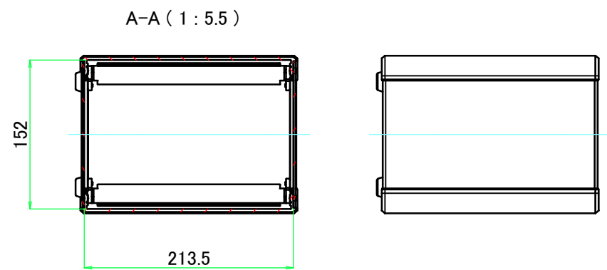
D view
